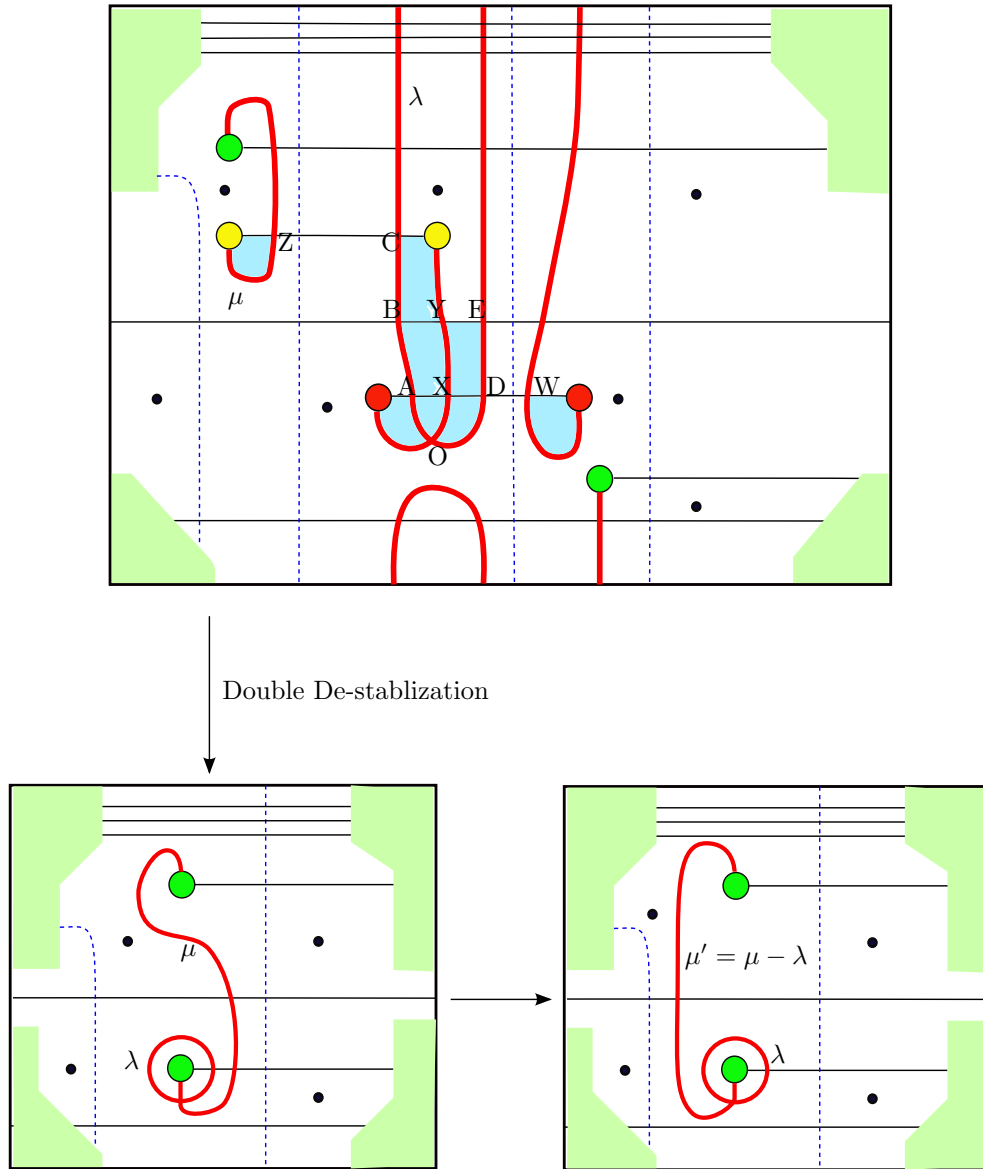
FIGURE 3. Special Heegaard diagrams for knot complements are the union of the genus 4 surface \Sigma_1 with boundary illustrated as the white part of the figure on top with another surface with boundary. The curves \lambda and \mu are illustrated as bold red curves, while \alpha \cap \Sigma_1 and \beta \cap \Sigma_1 are denoted by black curves and dashed blue curves, respectively. The intersection of \mu and \lambda is denoted by O and some of the intersection points in \alpha \cap (\lambda \cup \mu) are labeled (by A, B, C, D, E, X, Y, Z and W ). Double Destabilization and a change in the framing (equivalently, in the parametrization of the boundary torus) gives the two Heegaard diagrams on the bottom of the figure.
