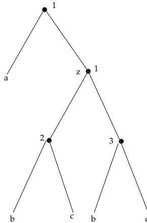
Figure 1: Tree implementing f
